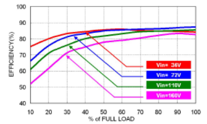
43RHK10-110S24W Efficiency vs. Output Load
