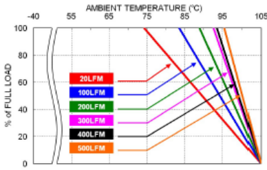
43RHK10-110S24W Derating Curve
