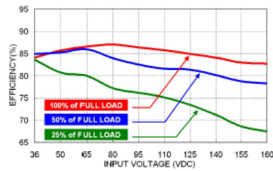
43RHK10-110S24W Efficiency vs. Input Voltage
